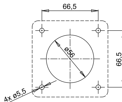
Fixing template
